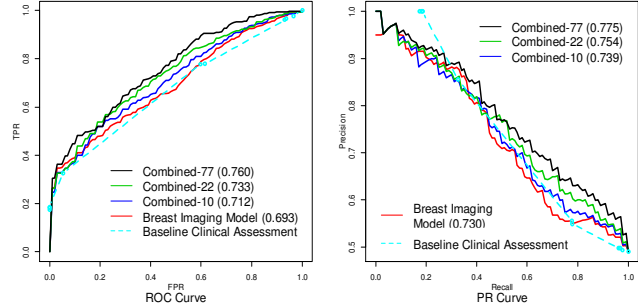
Figure 1. The ROC curves and PR curves for the baseline clinical assessment, the Breast Imaging model the three combined models.
